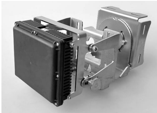
Bracket, exemplarily attached to a sensor
