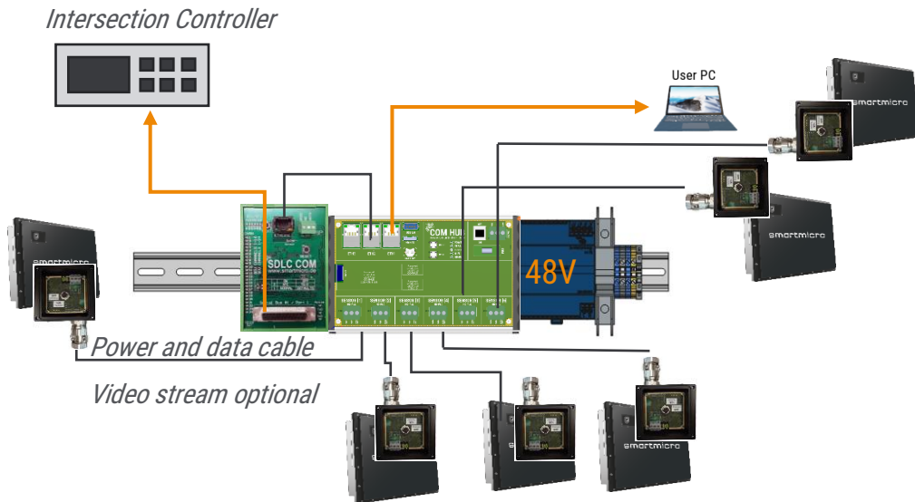
Figure 2-1 Connecting six smartmicro sensors to a controller through the COM HUB and SDLC Module
