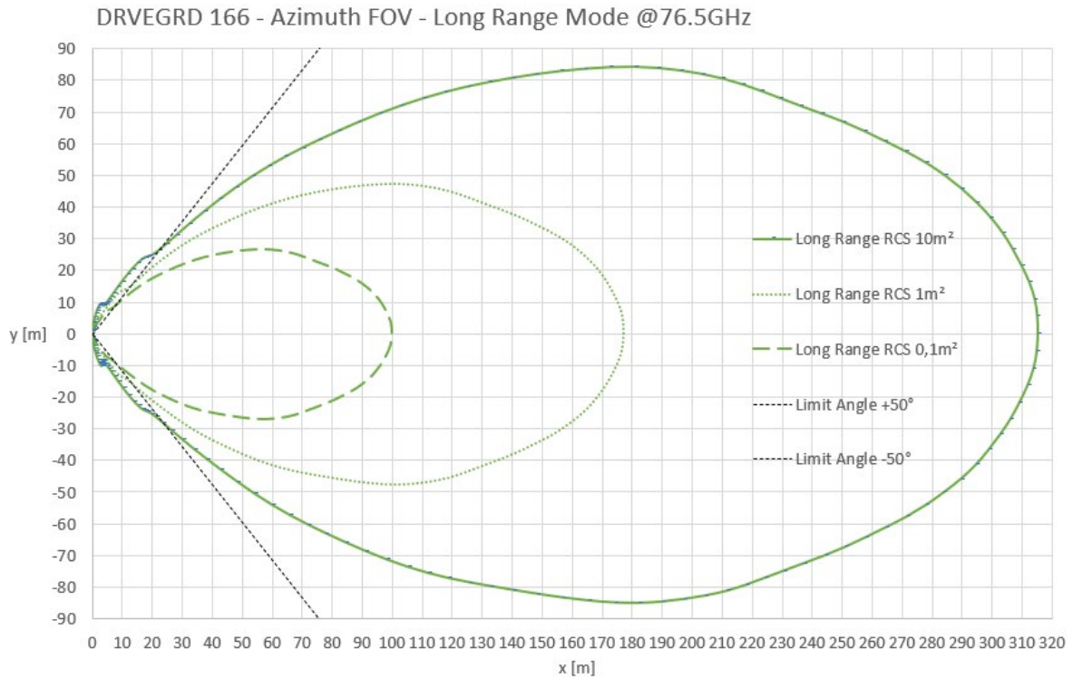
Figure 1: Field of view Azimuth Plot Long-Range Mode
