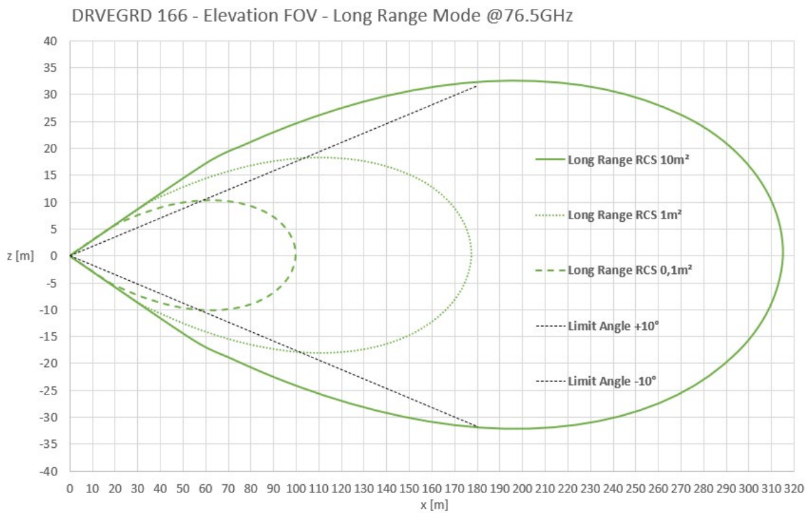
Figure 2: Field of view Elevation Plot Long-Range Mode
