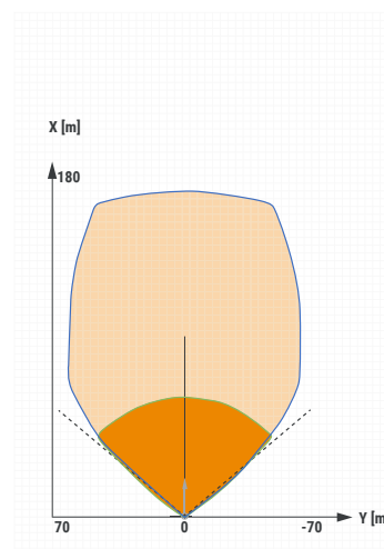
DRVEGRD ® 152 Azimuth Beam — Long-Range Mode (10m 2 Target) — Medium-Range Mode (10m 2 Target) --- Field Of View Limits
