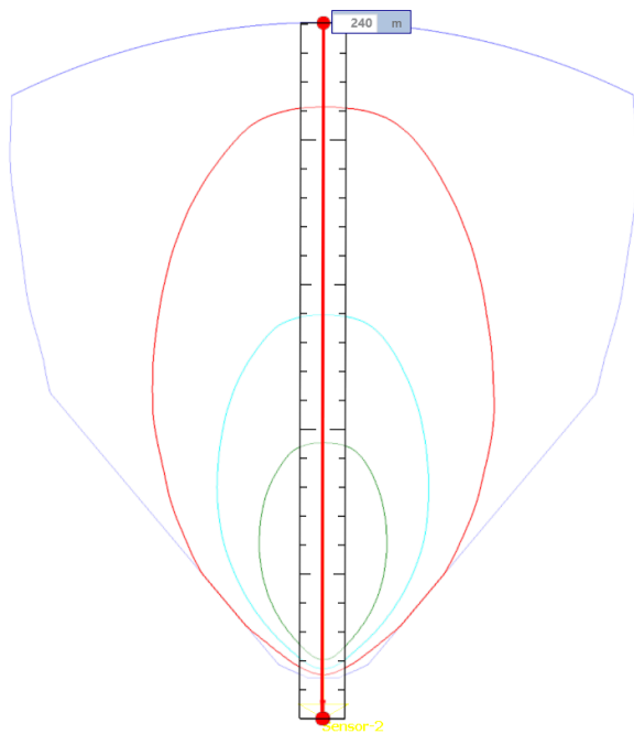
Beam for x-long-range mode (waveform 2)
