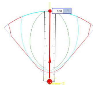
Beam for x-medium-range mode (waveform 3)
