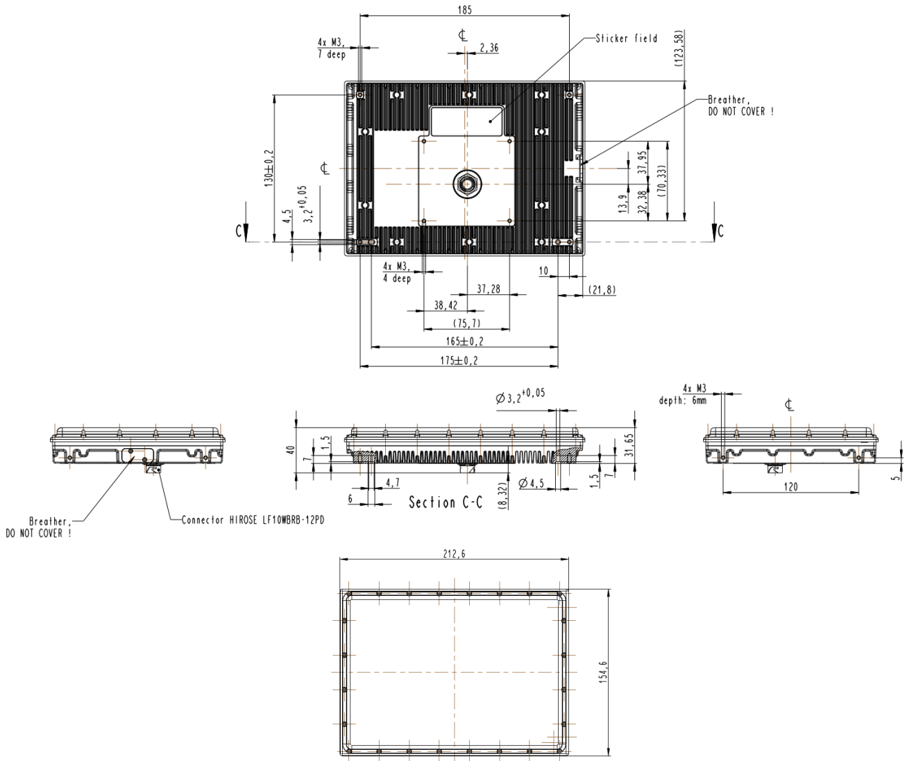
Figure 7: Sensor Dimensions.
