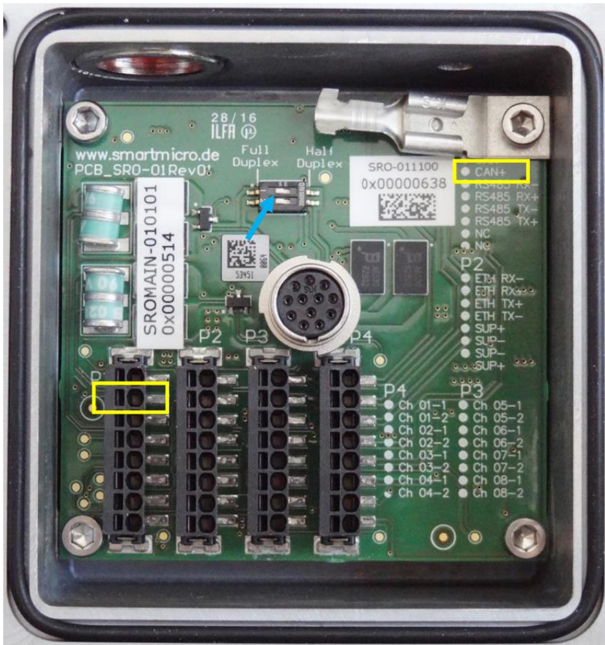
Figure 5: SRO-01xxxx pinout and jumpers
