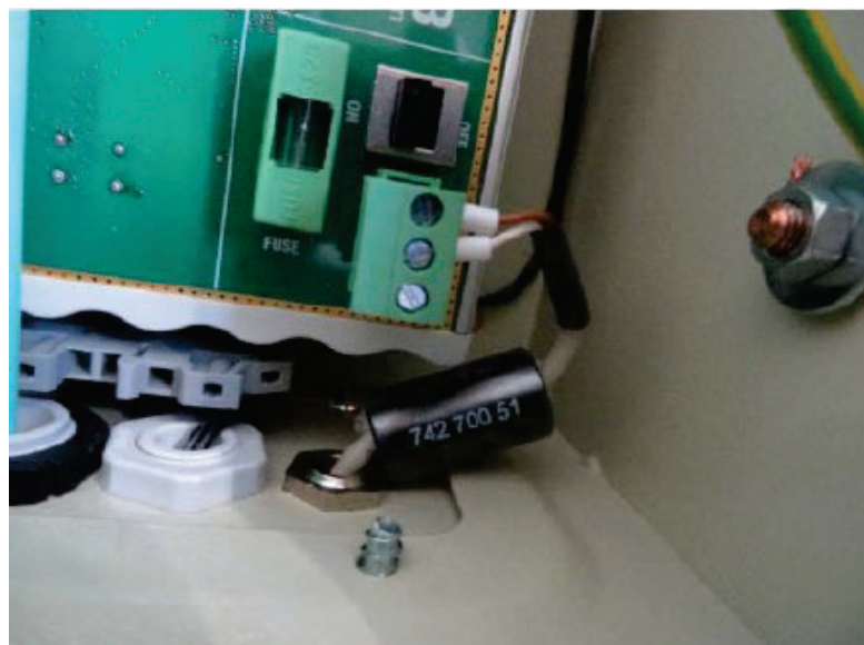
Ferrites 742 700 51 on the DC Power terminals of the COM HUB
