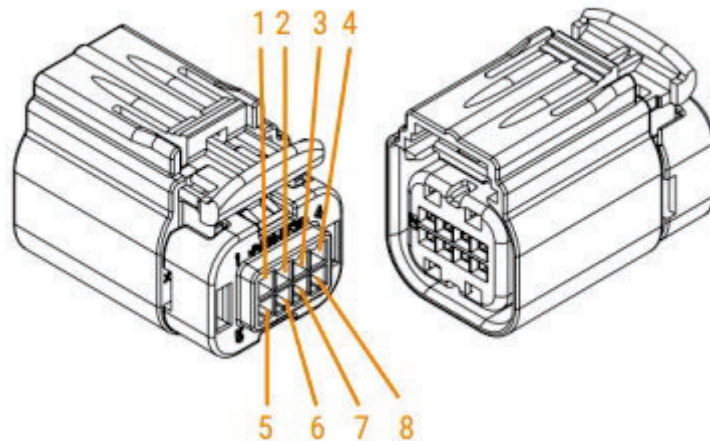
View on solder cup side of socket showing the pin numbering (rear view of female counterpart to be connected to sensor)
