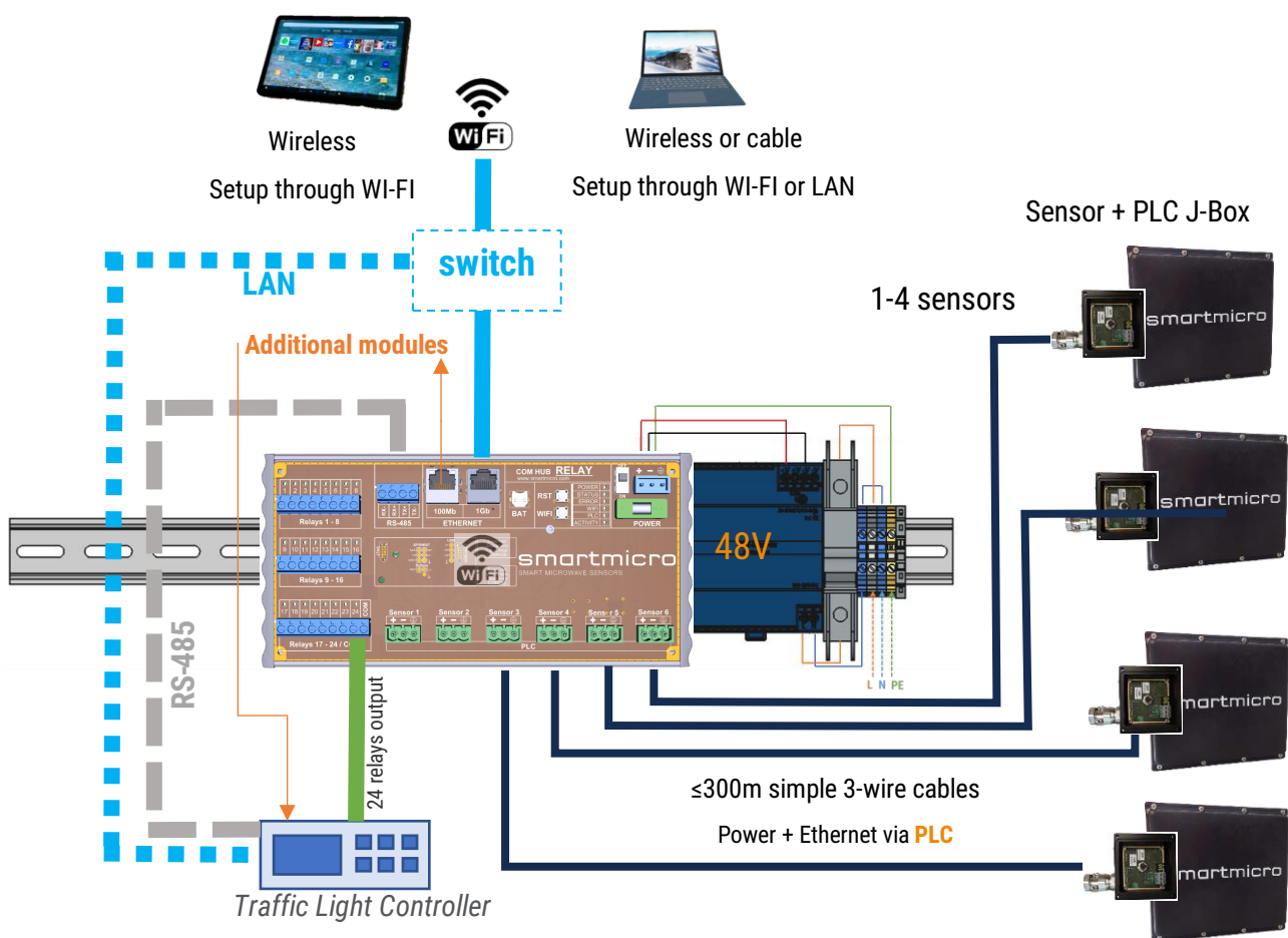
Connecting smartmicro sensors to a controller through COM HUB Relay 24
